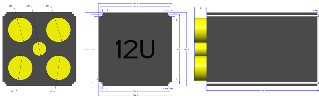
CubeSat 12U Envelope
