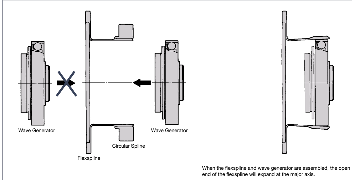
Assembly order for basic three elements
