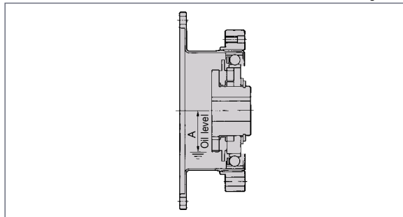
Oil level for horizontal use
