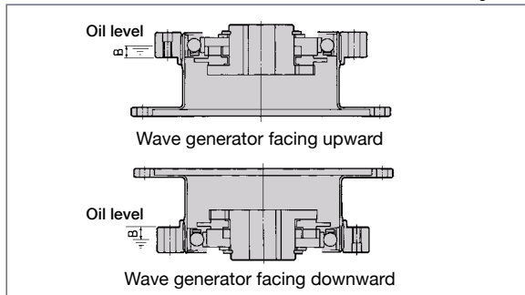
Oil level for vertical use
