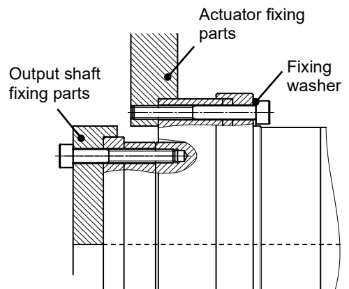
Assembly example 2
