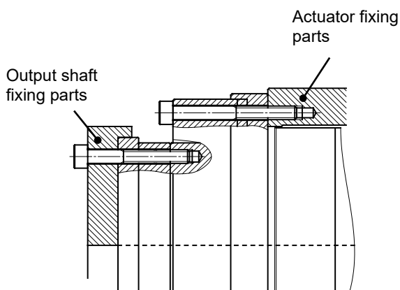
Assembly example 1
