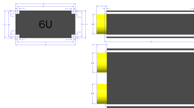
CubeSat 6U Envelope
