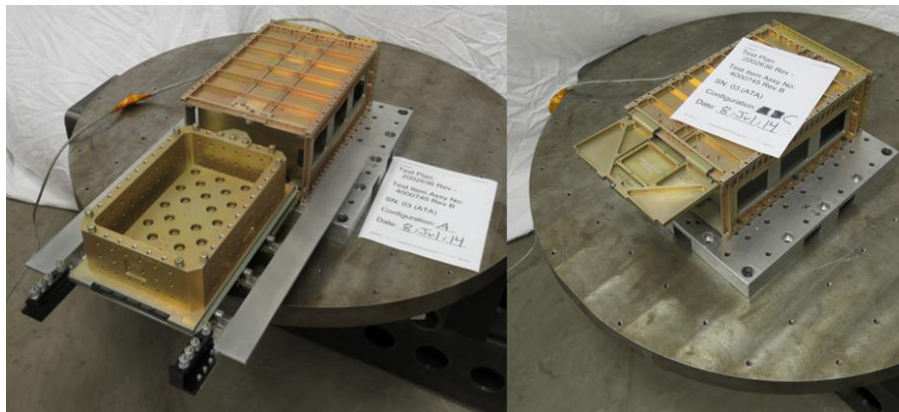
Figure 24-14: CSD mounted via -Y and +Y faces
