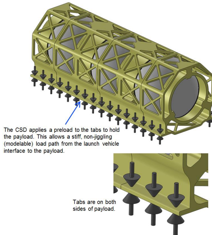
Figure 3-3: Preloaded tabs of a 3U payload (ref. 2)
