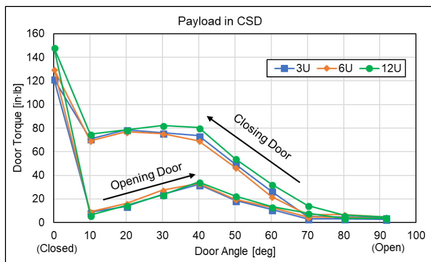
Figure 16-4: CSD door torque with payload installed
