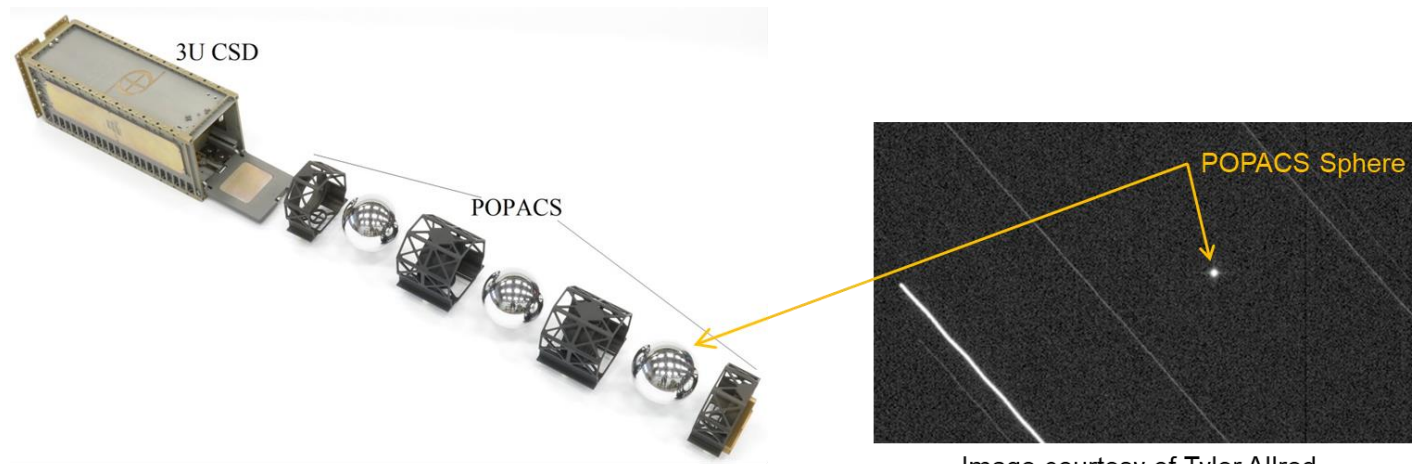
Figure 1-2: POPACS satellite and on-orbit image
