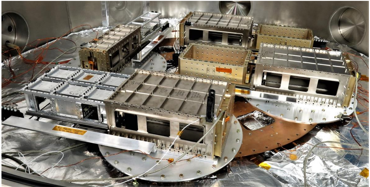
Figure 12-3: Thermal vacuum testing 4 CSDs in PSC's chamber. Conveyors allow complete payload dispensing (see Section 25).
