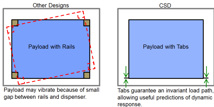
Figure 3-2: Benefit of tabs vs. rails
