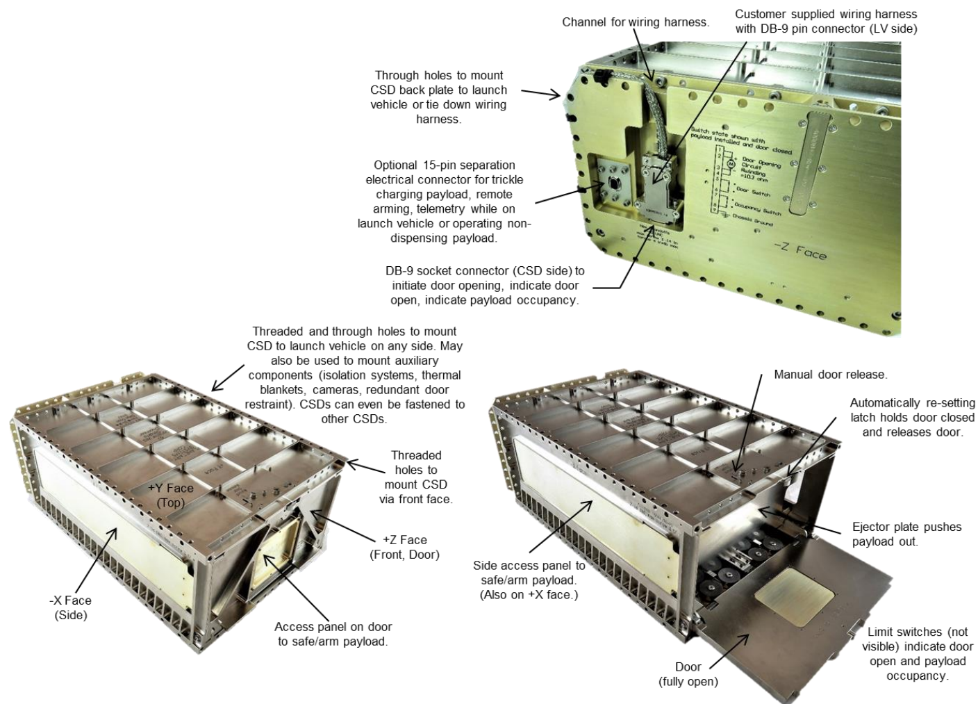
Figure 2-1: CSD features (6U shown)
