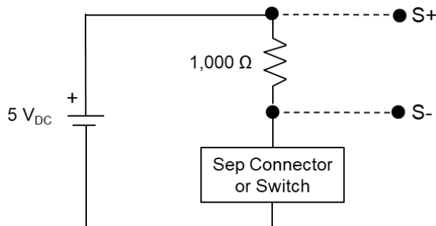
Figure 7-3: Measurement circuit
