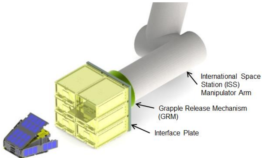
Figure 24-9: ISS manipulator arm dispensing six 6U payloads
