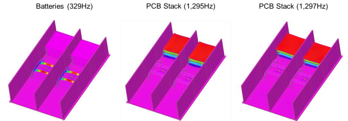
Figure 3-6: Normal modes analysis of satellite elements
