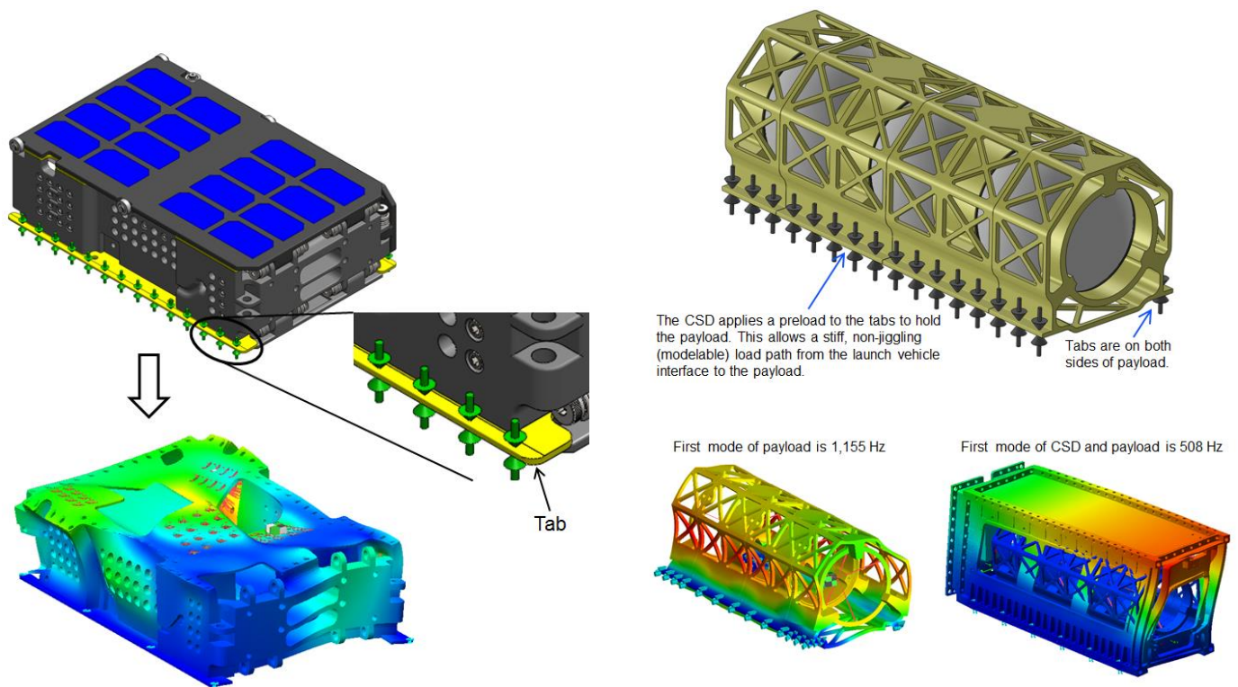
Figure 9-2: Prediction of 6U dynamic response
