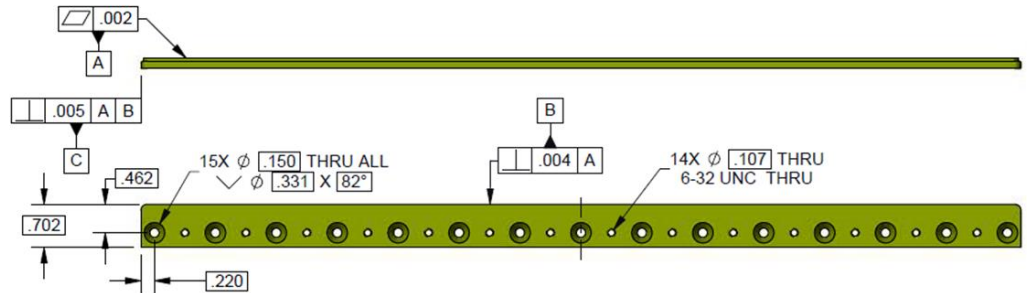
Figure 11-2: Example bolt-on tab drawing
