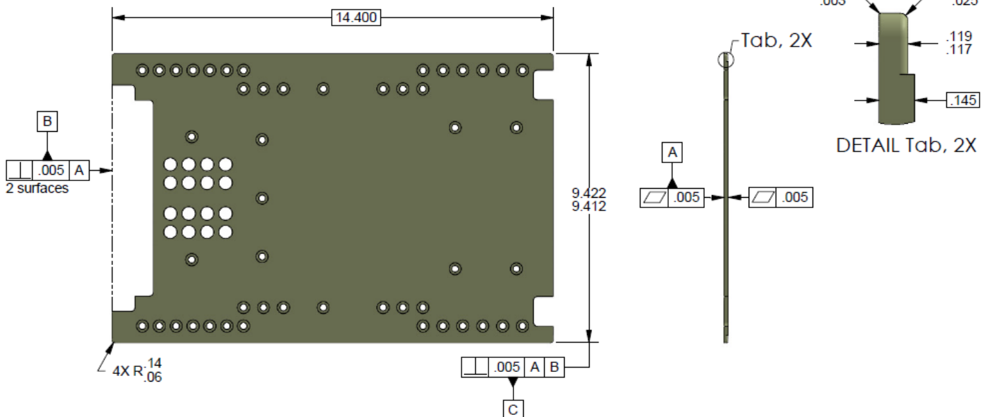
Figure 11-1: An example tab plate production drawing
