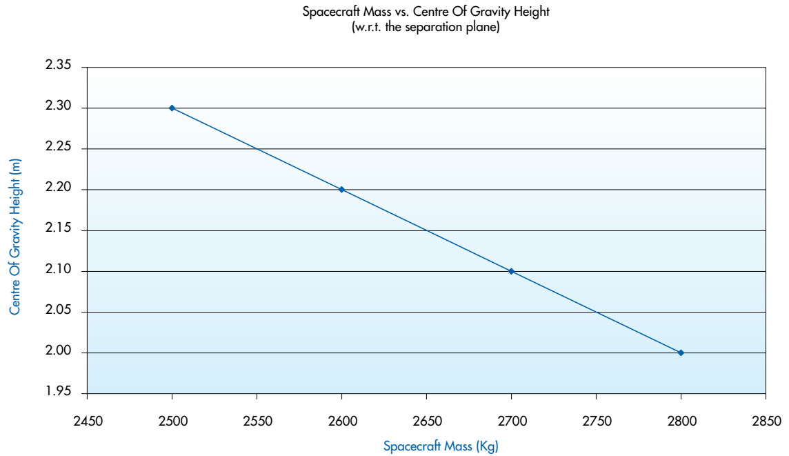
Figure A 2 - 8: Limit Loads for Adapter 1194-SF
