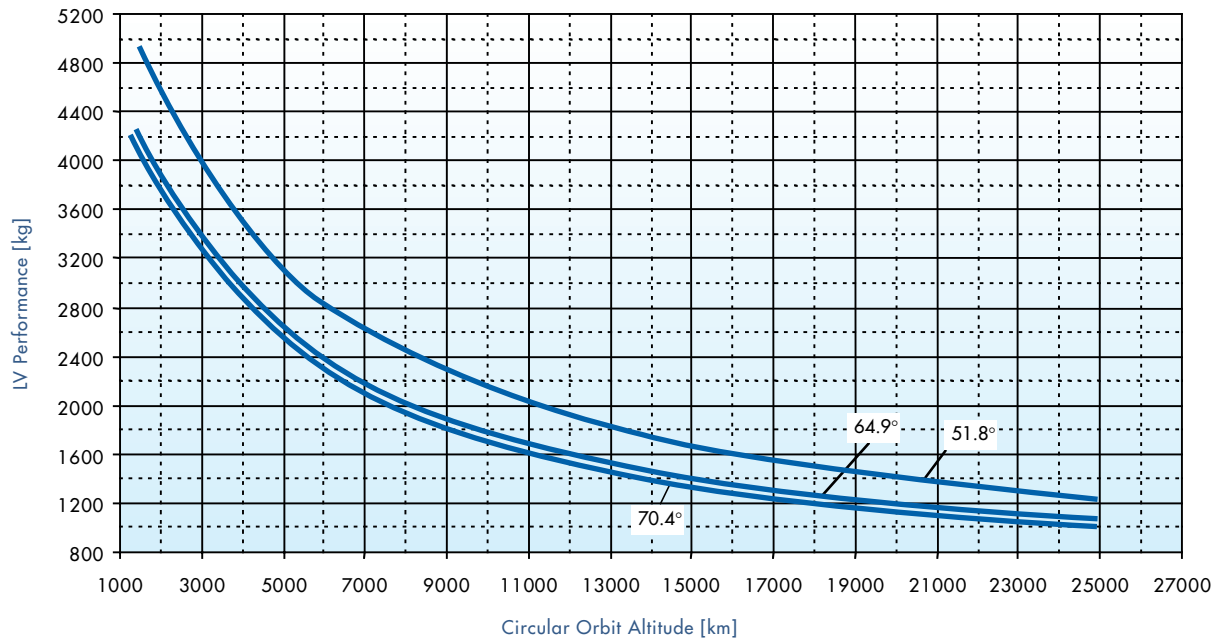
Figure 2-9: LV Performance for Medium Circular Orbits: H_{circ} = 1500\text{--}25,000\text{ km}
