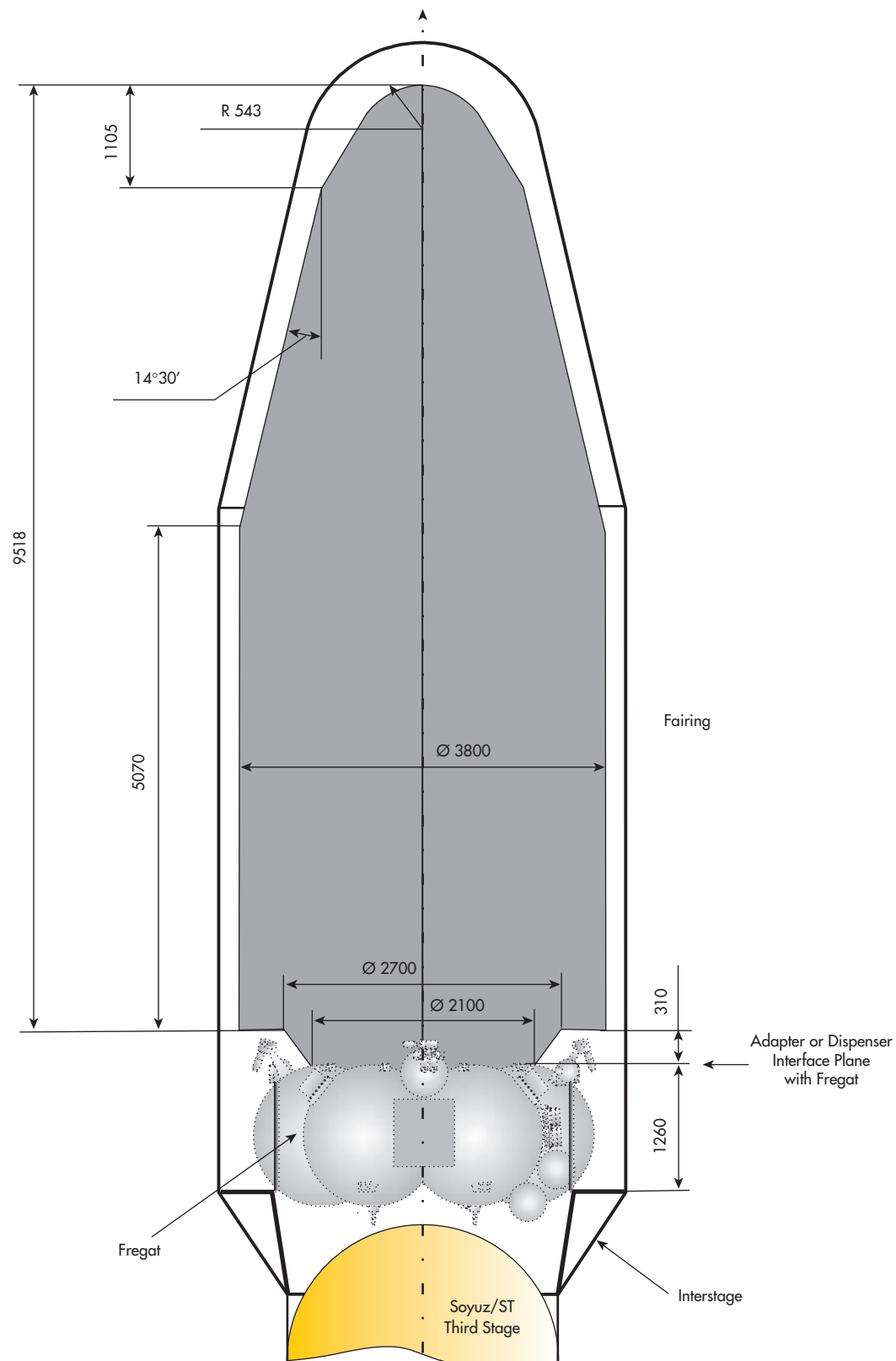
Figure 5-2: Fairing Type ST: Spacecraft-Stack Allocated Volume
