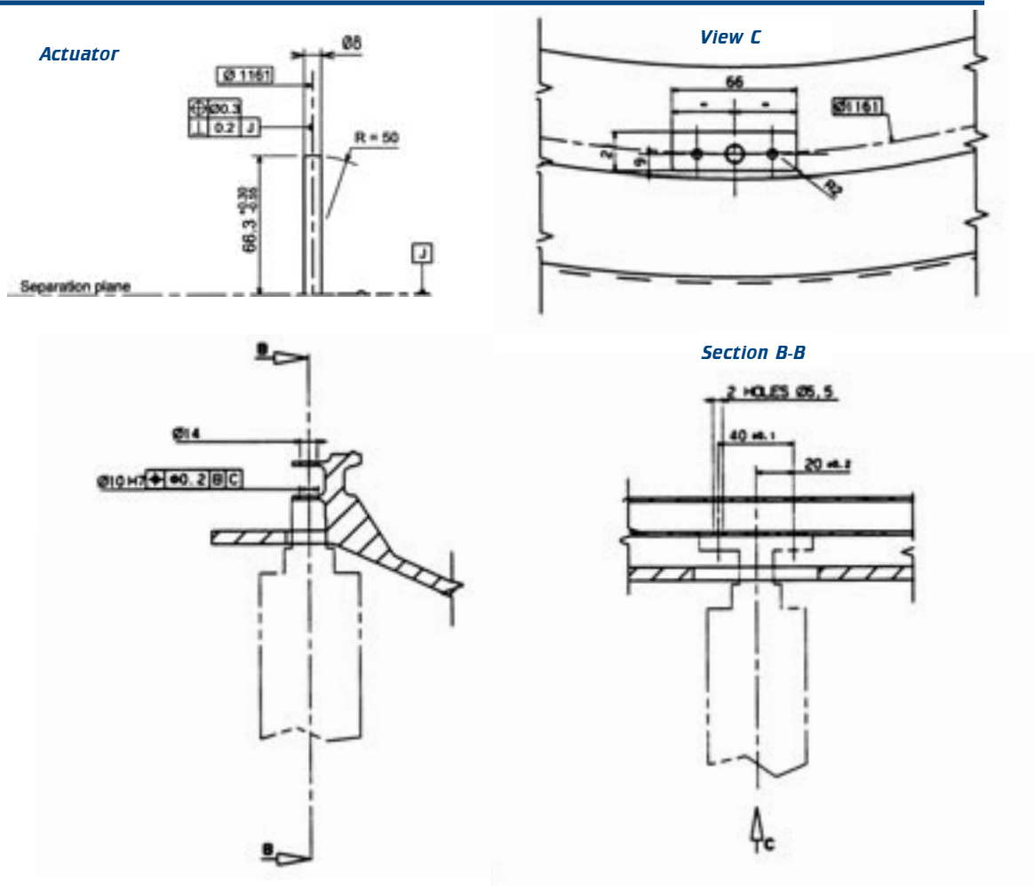
Figure A 2 - 7: Spring Actuator Design
