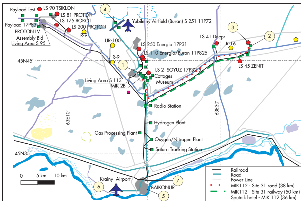
Figure 6-2: Baikonur Cosmodrome
