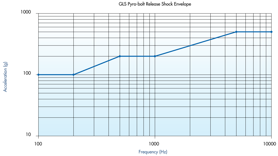
Figure A 2 - 14: GLS Dispenser Pyro-Bolt Release Shock Spectrum at Dispenser/Spacecraft Interface
