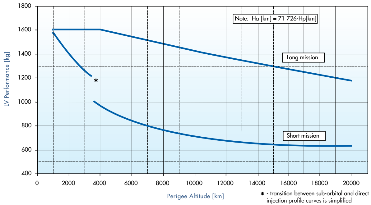
Figure 2-16: LV Performance for a 24-Hour Molniya-Type Orbit: H_{\text{perigee}} = 1000\text{--}20,000\text{ km}
