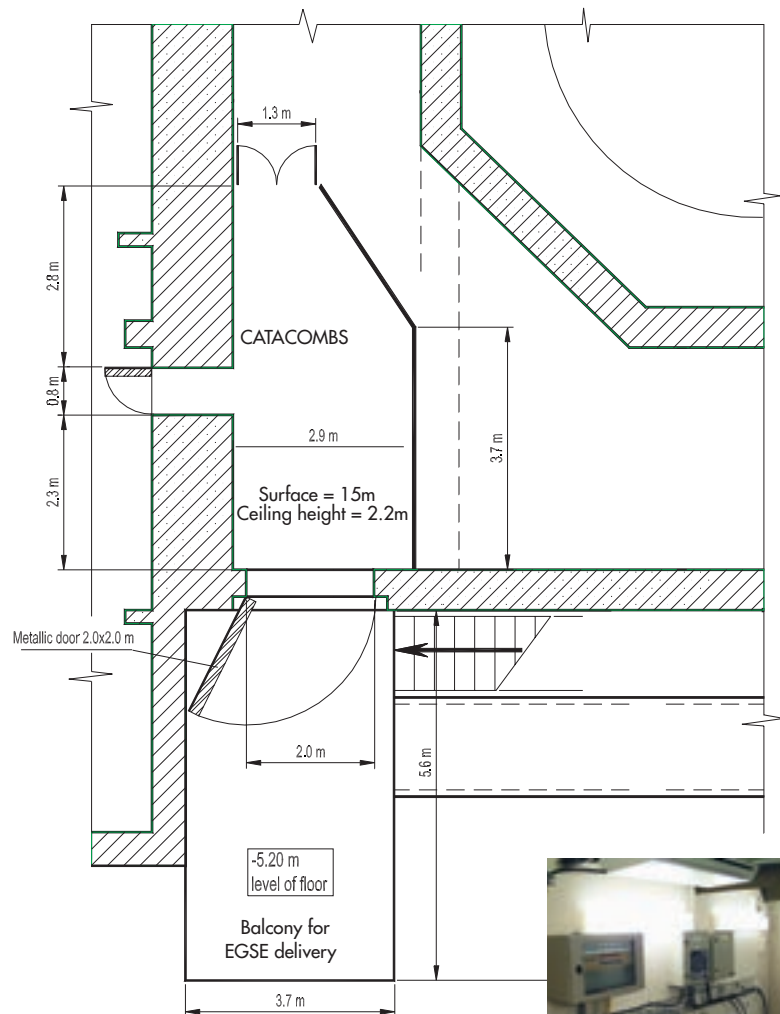
Figure 6-11: Catacombs Layout
