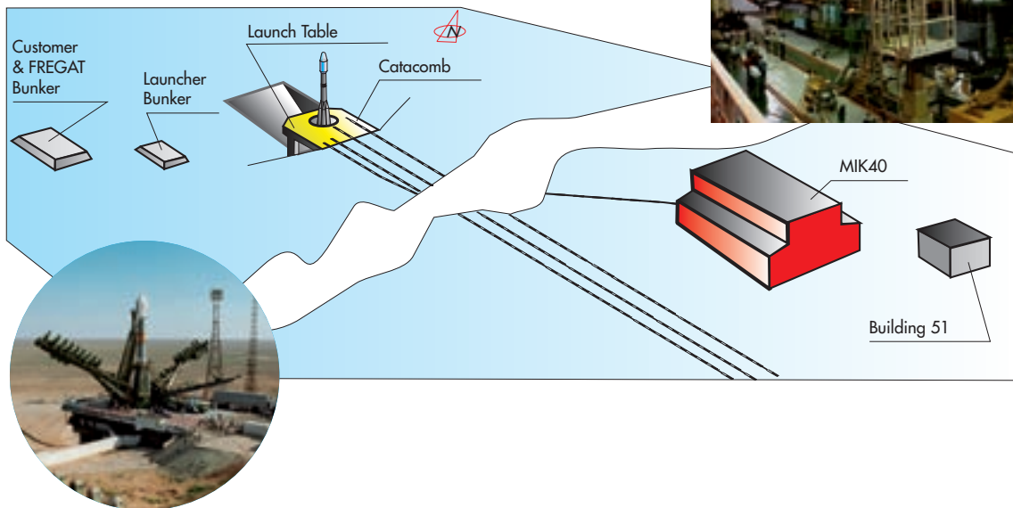
Figure 6-4: Site 31 Layout
