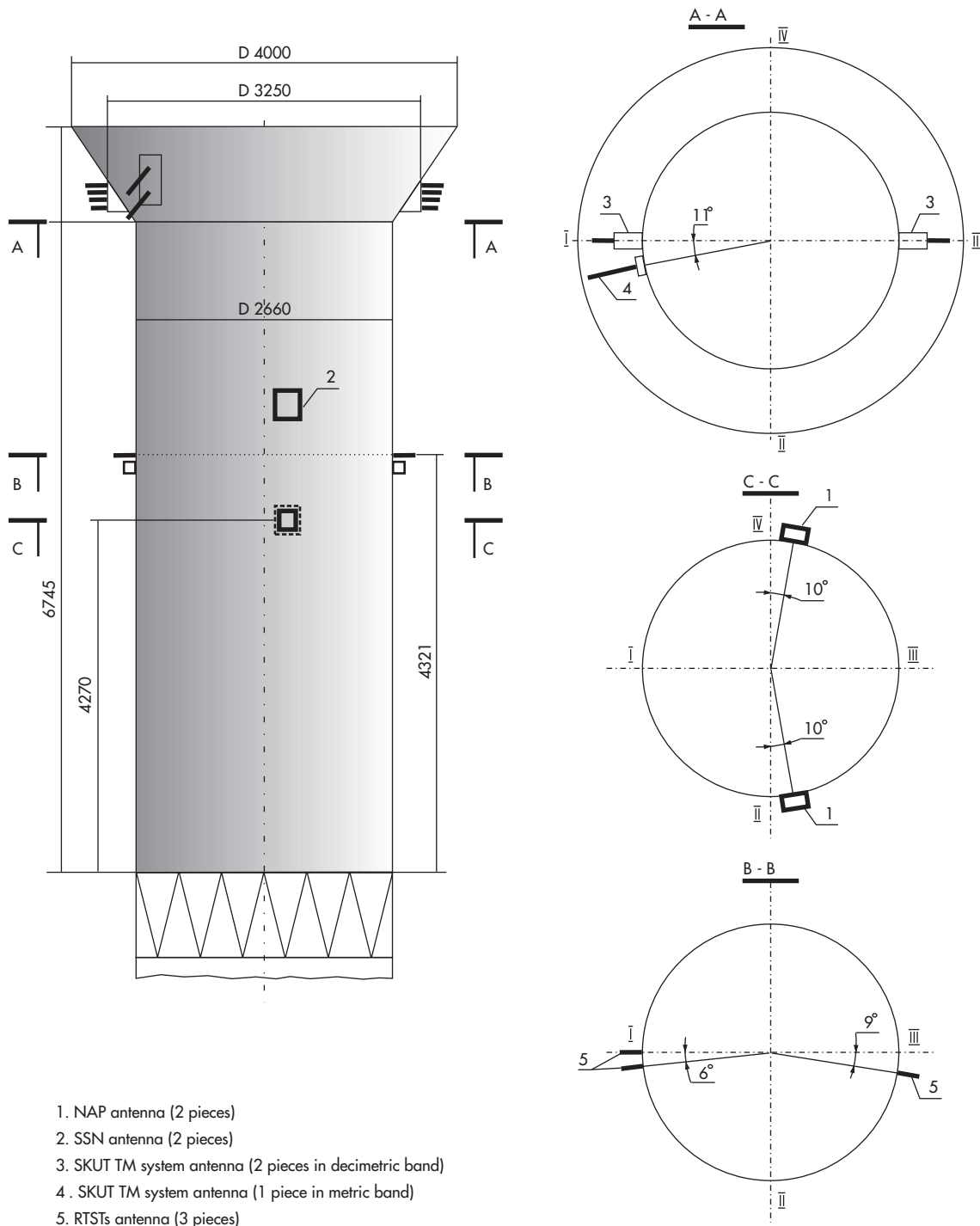
Figure 3-6: Third-Stage Soyuz/ST – Location of Antennas
