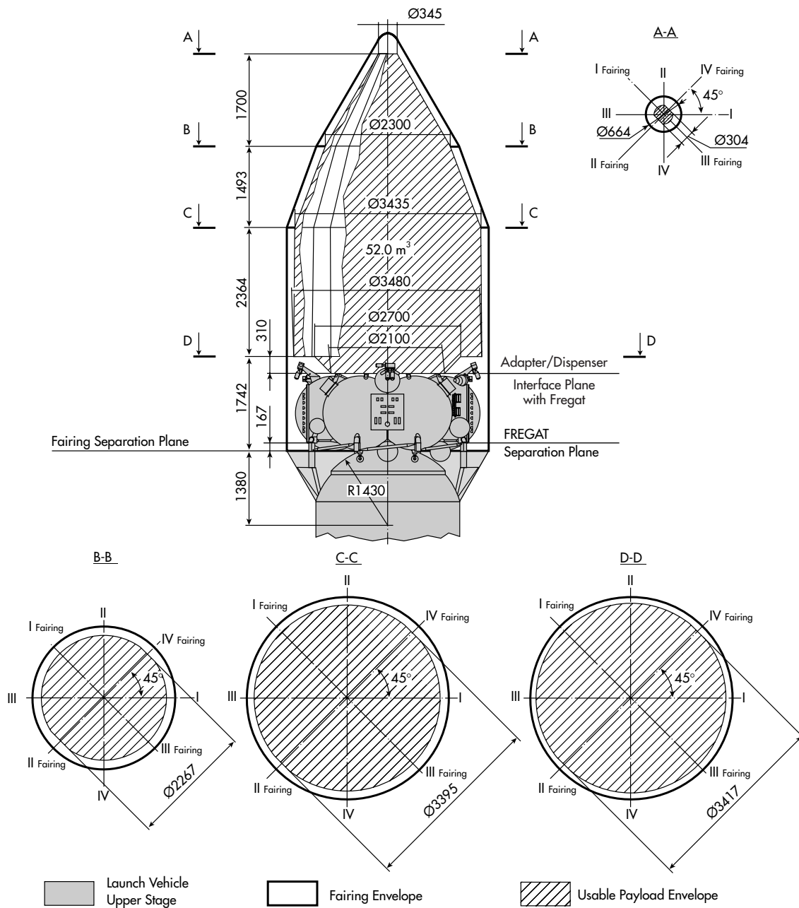
Figure 5-4: Fairing Type S: Spacecraft-Stack Allocated Volume
