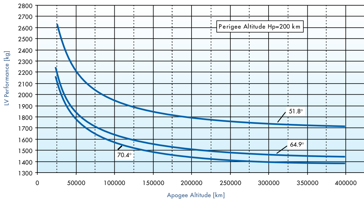
Figure 2-17: LV Performance for High Elliptical Orbit: H_{\text{apogee}} = 25,000\text{--}400,000\text{ km}
