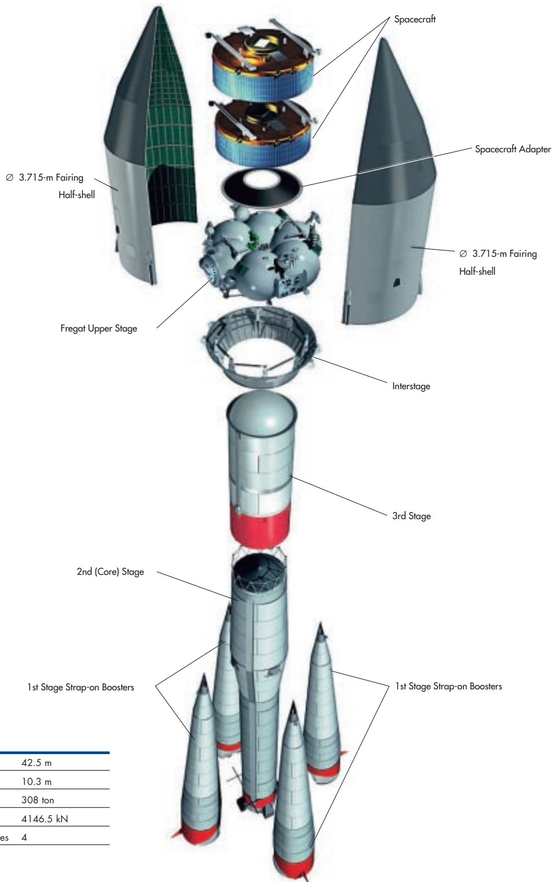
Figure 1-1: Soyuz Configuration
