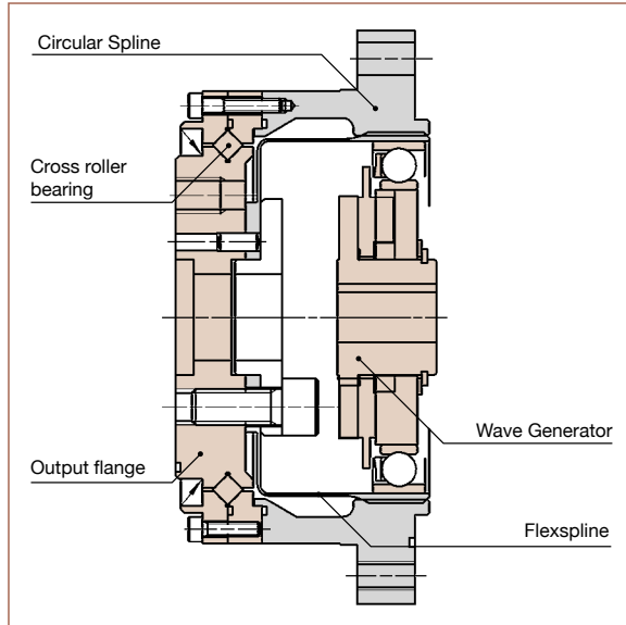
Structure of CSG/CSF series gear unit
