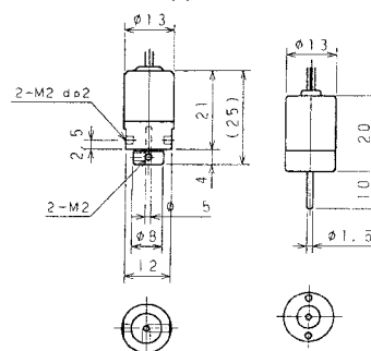
Appearance
