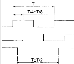
Output Waveform
