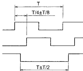
Output Waveform
