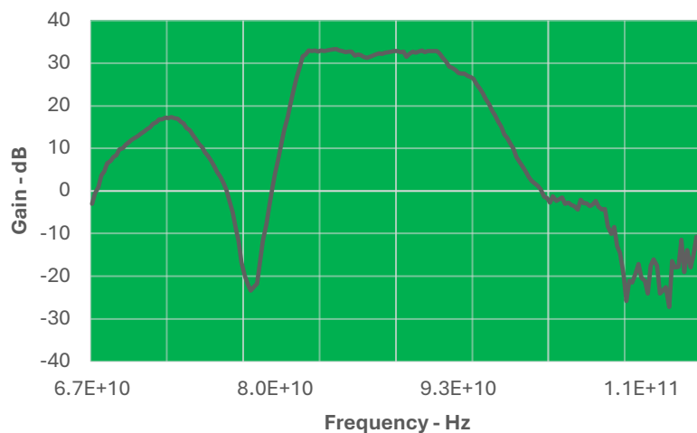
WB-LNA-86 Gain Plot
