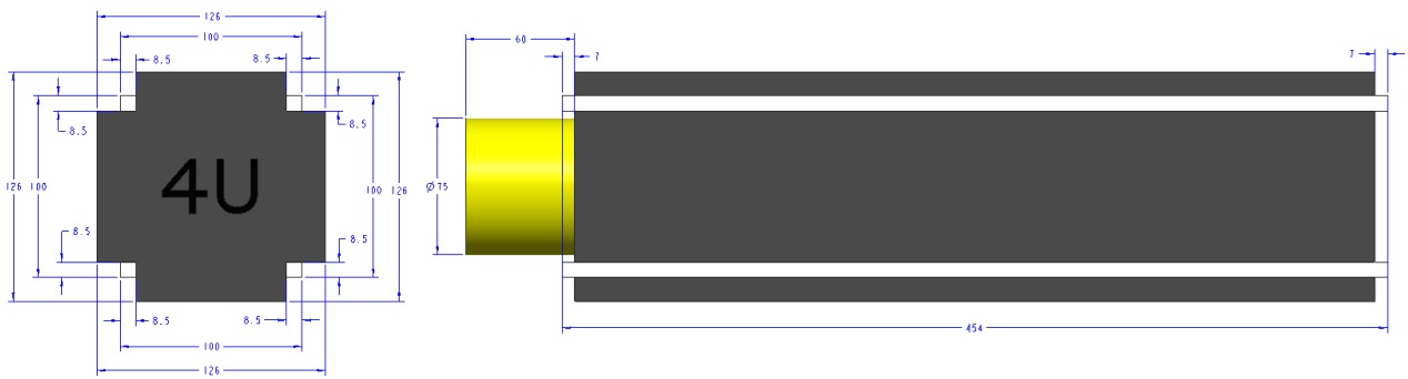
CubeSat 4U Envelope
