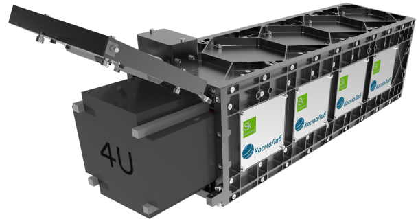
CubeSat 4U Placement
