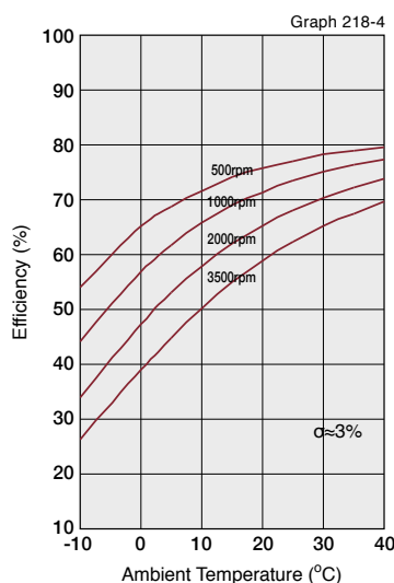
Size 17 to 50/ Ratio 80, 100, 120
